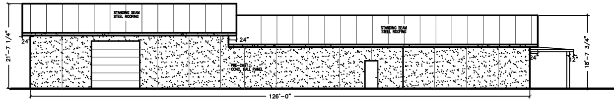
SOUTH ELEVATION
