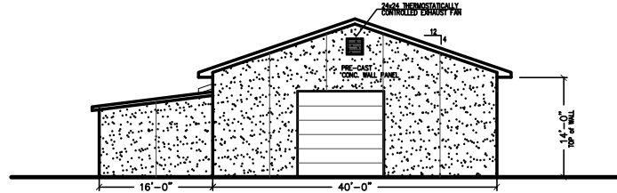
EAST ELEVATION
